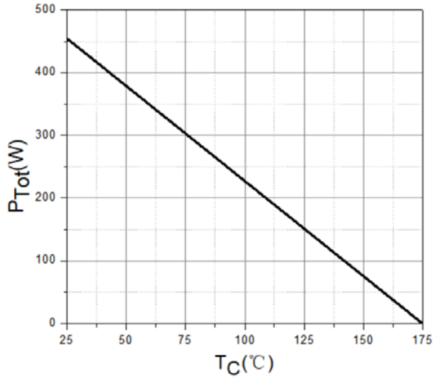
Figure 6. Power Derating
